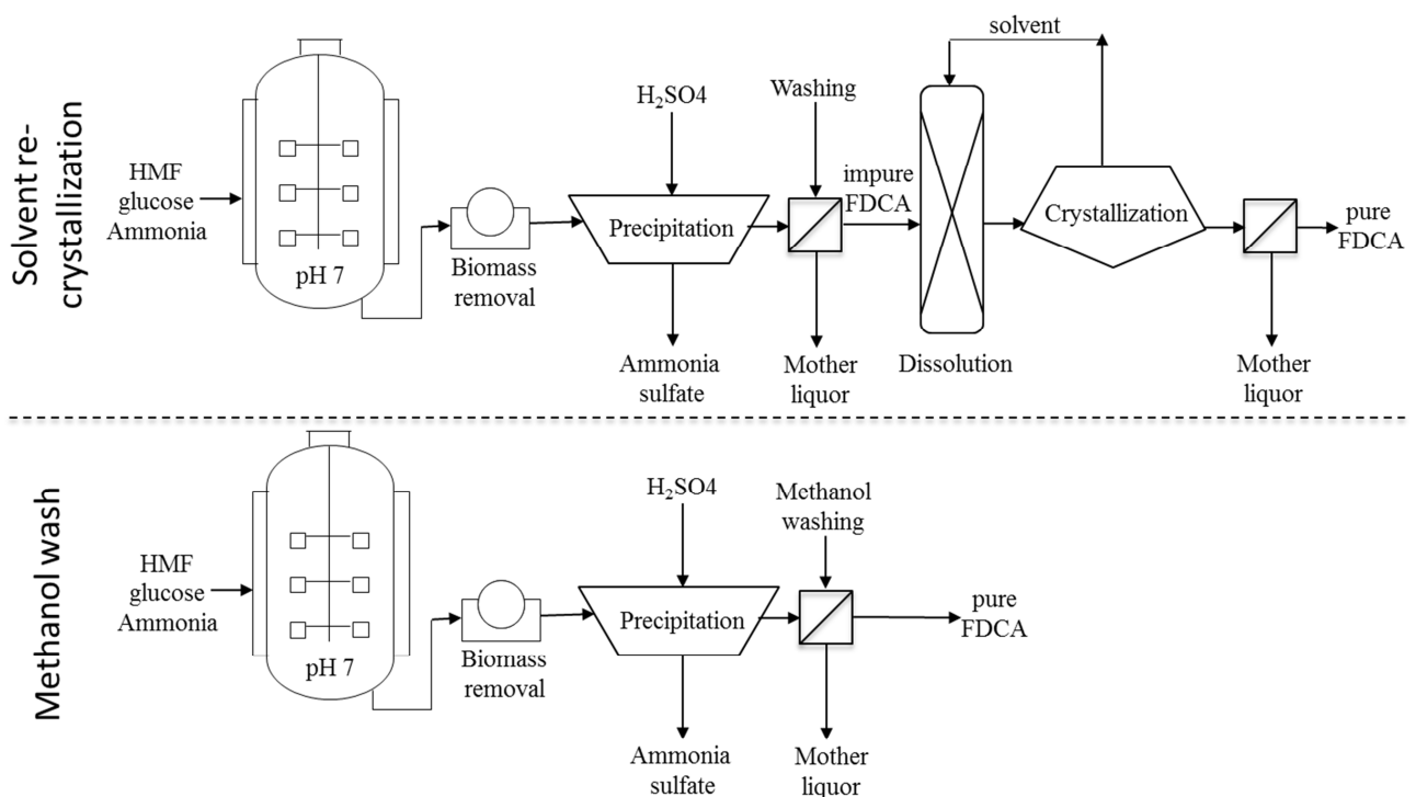
Figure 6: Process options evaluated for further process selection to produce FDCA at pilot scale (in the solvent re-crystallization option, 2 solvents were considered: DMSO and super heat water)
